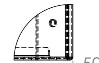
DETAIL B SCALE 1 : 5
