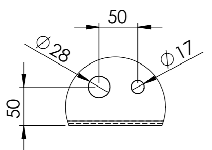
DETAIL C SCALE 1 : 5
