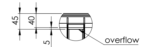
DETAIL A SCALE 1 : 5
