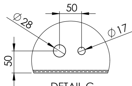
DETAIL C SCALE 1 : 5
