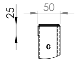
DETAIL A SCALE 1 : 5
